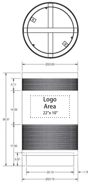
Dimensions represent can only lid accounted for separately
